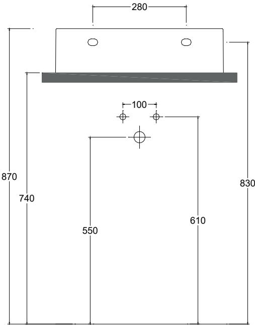
Vista posteriore Back view
